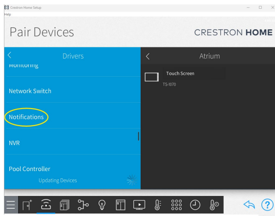
Figure 12 Notifications
