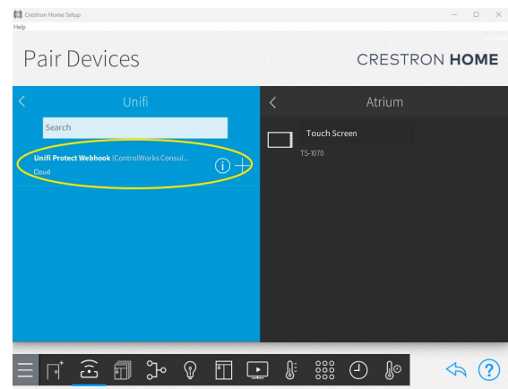
Figure 13 – Unifi
