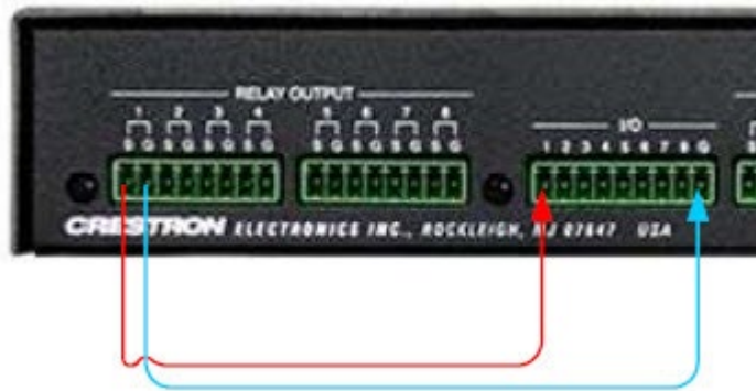
Figure 8 - CP4-R Relay Wiring
