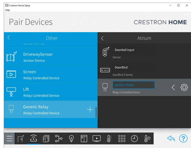
Figure 6 - Adding Relay
