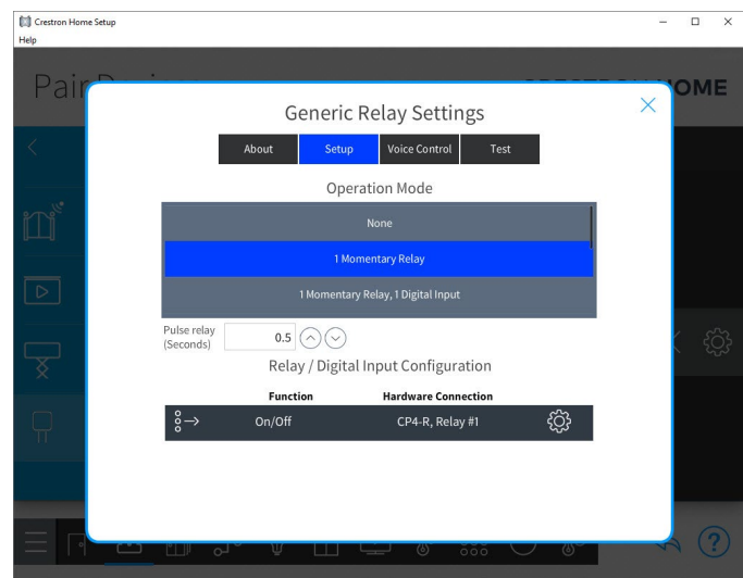
Figure 7 - Relay Setup
