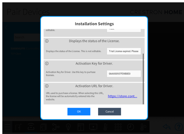
Figure 17 - License
