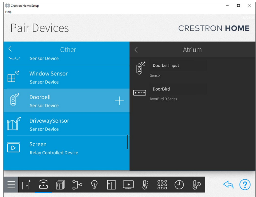
Figure 5 - Add Doorbell
