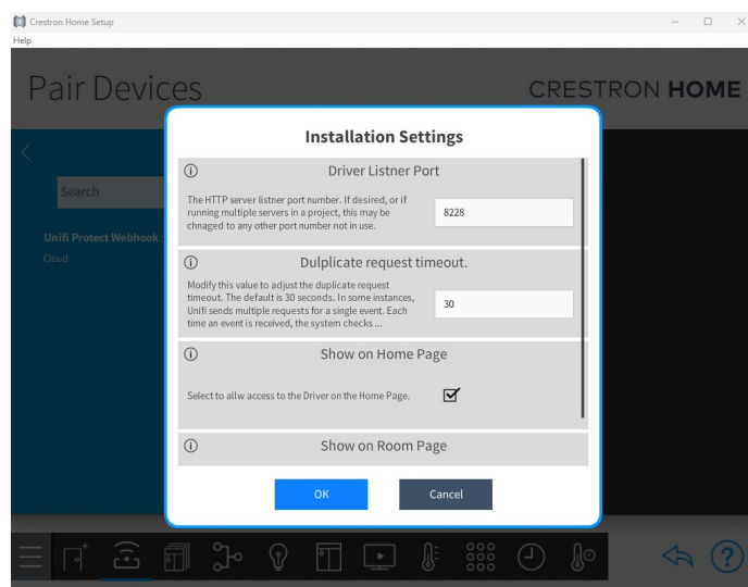
Figure 16 - Installation Settings
