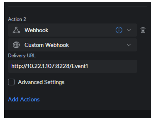
Figure 3 - Setup Action
