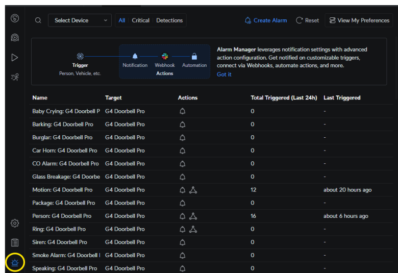
Figure 1 - Alarm Manager
