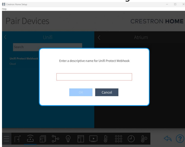
Figure 14 - Name Device
