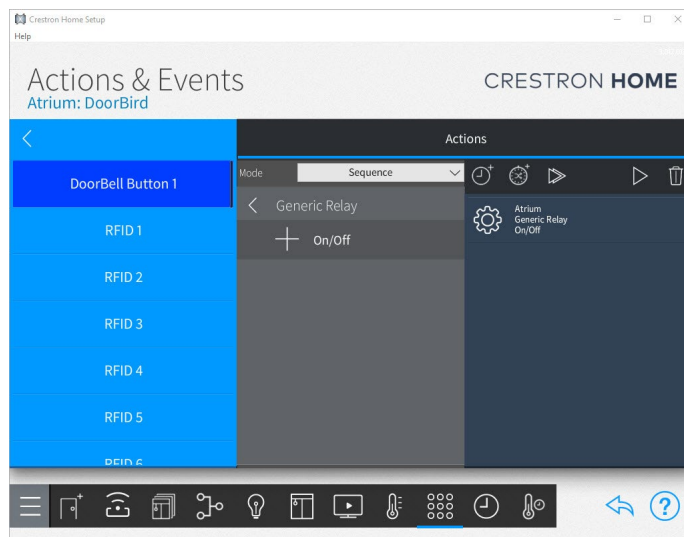
Figure 26 - Connecting DoorBird Event to Relay
