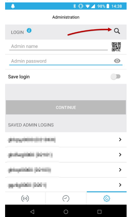
Figure 6 - Device Discovery
