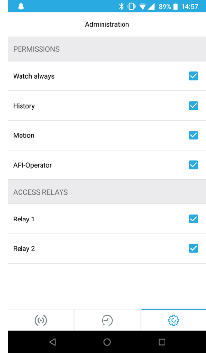
Figure 8 - Selecting Permissions
